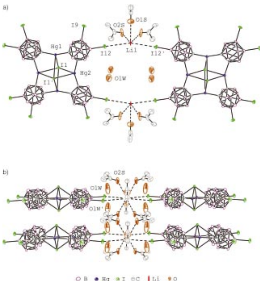
Figure 2. Crystal packing representation of [\text{Li}_2\{(\text{CH}_3)_2\text{CO}\}_6][\mathbf{1} \cdot \text{I}_2] \cdot 4\text{H}_2\text{O} (ORTEP diagram; hydrogen atoms omitted for clarity). a) Projection perpendicular to the \text{Hg}_4 plane. b) Projection parallel to the \text{Hg}_4 plane. Selected interatomic distances [Å] and bond angles ^\circ : \text{I12} \cdots \text{Li1} 3.753, \text{Li1} \cdots \text{O1S} 3.114, \text{Li1} \cdots \text{O2S} 3.20(4), \text{O1W} \cdots \text{O1W'} 4.72(5); \text{I12} \cdots \text{Li1} \cdots \text{I12'} 162(1) .
